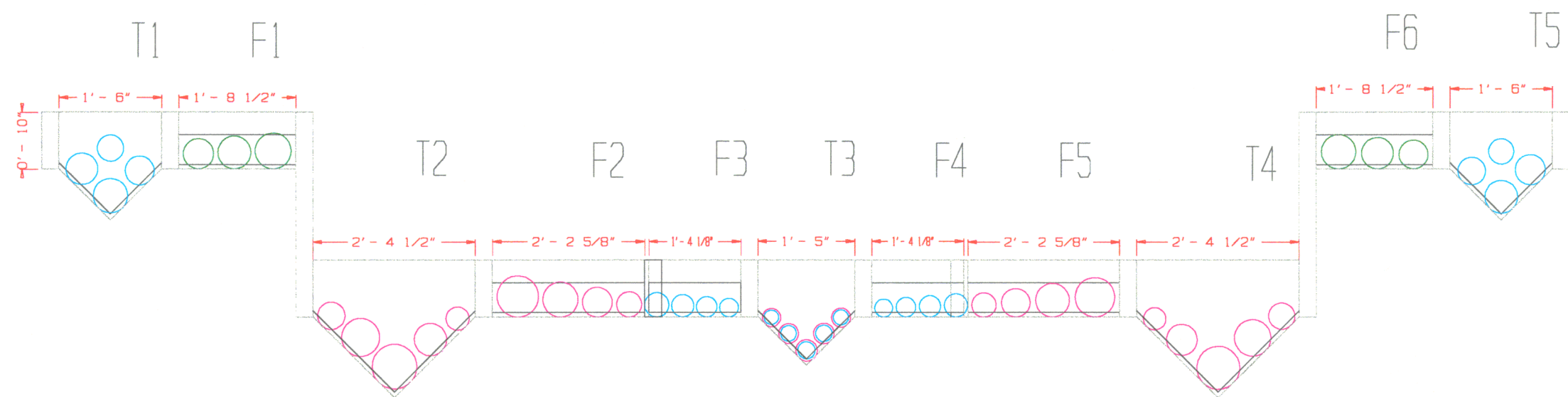
Plan View Sills/Case
